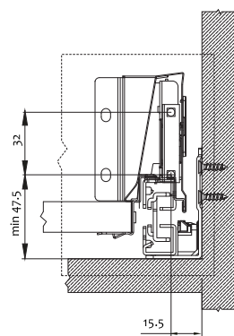
Front connector panel installation dimensions
