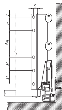
Back panel installation dimensions
