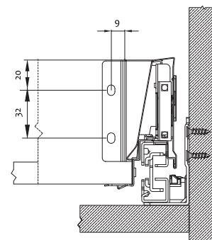
Back panel installation dimensions
