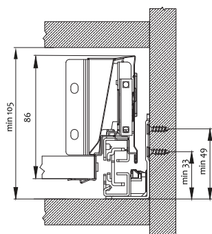
Cabinet space requirements
