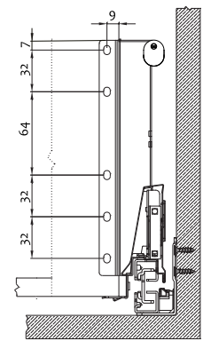
Back panel installation dimensions
