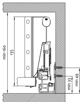
Cabinet space requirements
