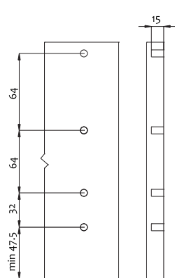
Front panel drilling dimensions
