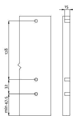
Front panel drilling dimensions
