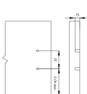
Front panel drilling dimensions
