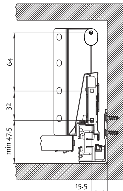
Front connector panel installation dimensions
